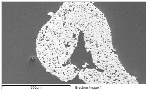
Figure 2 - An electron micrograph showing the highly sintered structure of STELEX ZR ULTRA
