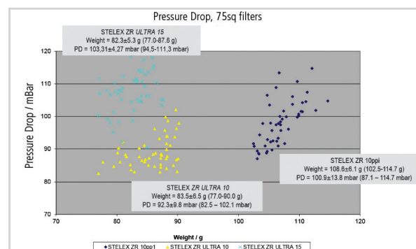
Figure 5 - The results of the pressure drop test
