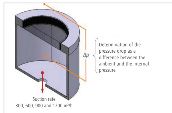
Figure 4 - A diagram showing the principles of the "Pressure Drop Tests"
